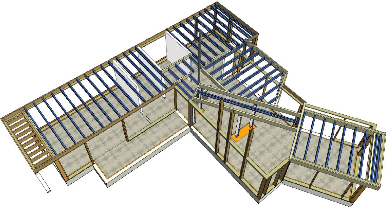
FLOOR STR 2 3D
